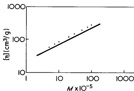
Figure 1 Predicted and experimental values of [\eta] for system A. ●, values calculated from equation (4); —, empirical curve
