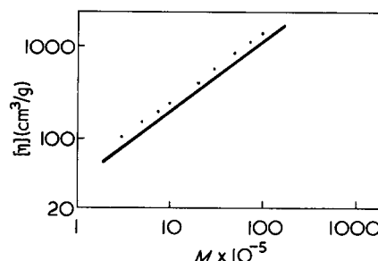
Figure 2 Predicted and experimental values of [\eta] for system B
