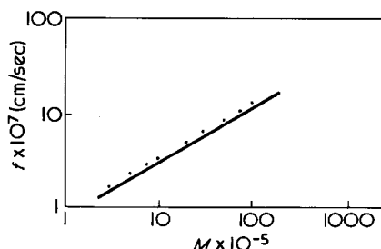
Figure 4 Predicted and experimental values of f for system B
