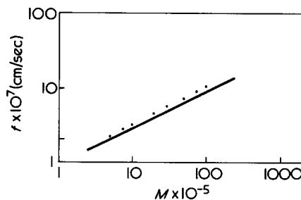
Figure 3 Predicted and experimental values of f for system A. ●, values calculated from equation (5); —, empirical curve
